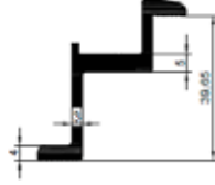
40'lik End Klemp 705 832 gr/m
